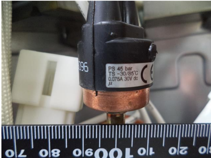
199. RAS-3M18U2AVG-E, High-Pressure Switch
