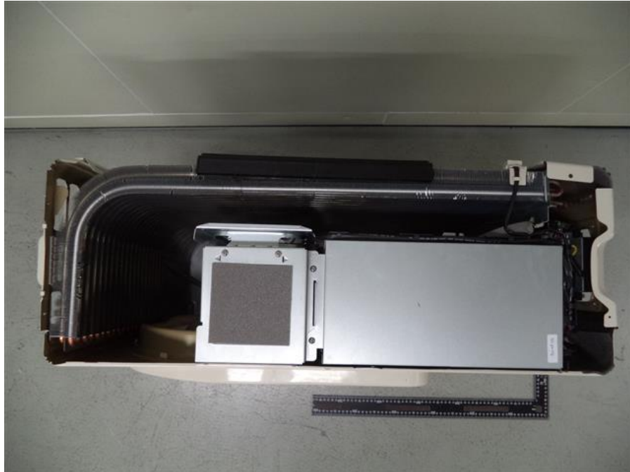
157. RAS-2M14U2AVG-E, Top view removed insulator
