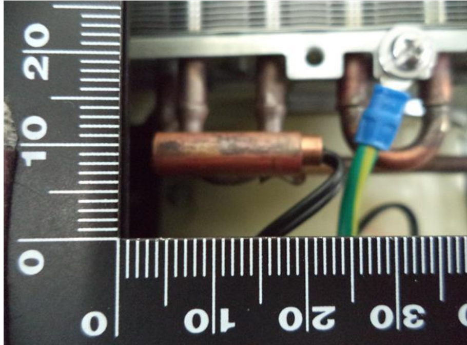
67. RAS-B07BKVG-E, Thermistor
