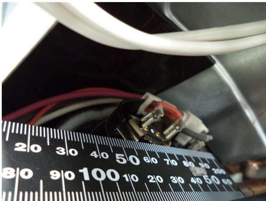
190. RAS-3M18U2AVG-E, Terminal of motor compressor and thermostat
