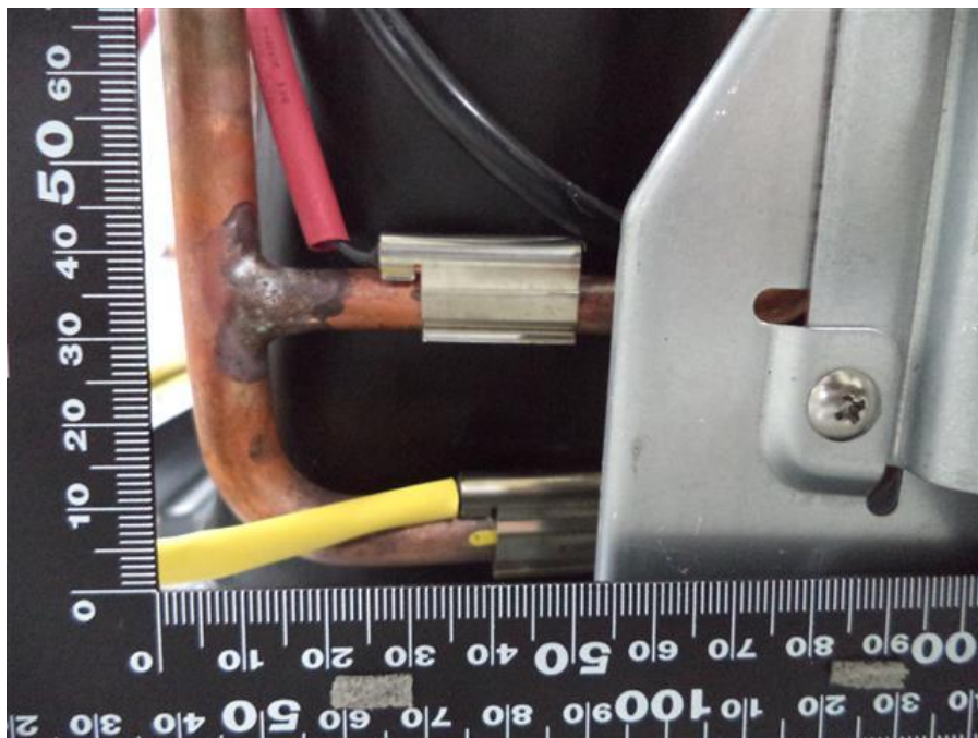
168. RAS-2M14U2AVG-E, Thermistor
