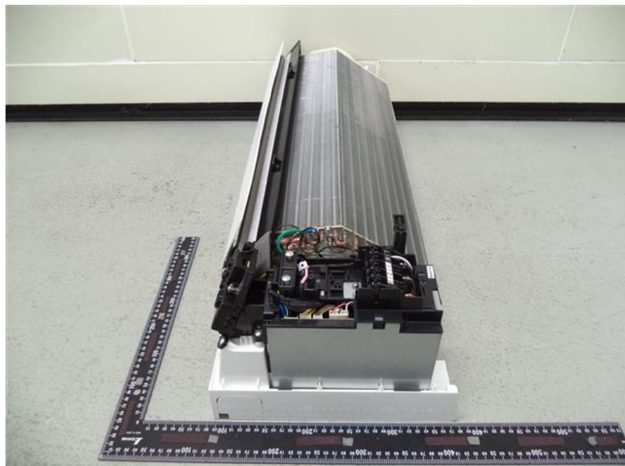
10. RAS-B10PKVSG-E, Internal right view
