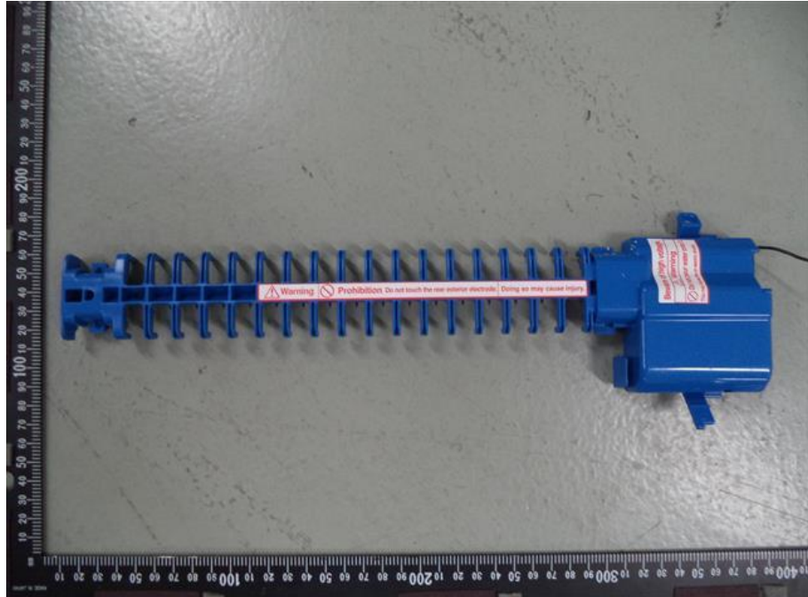
51. RAS-M10PKVPG-E, HV Generator
