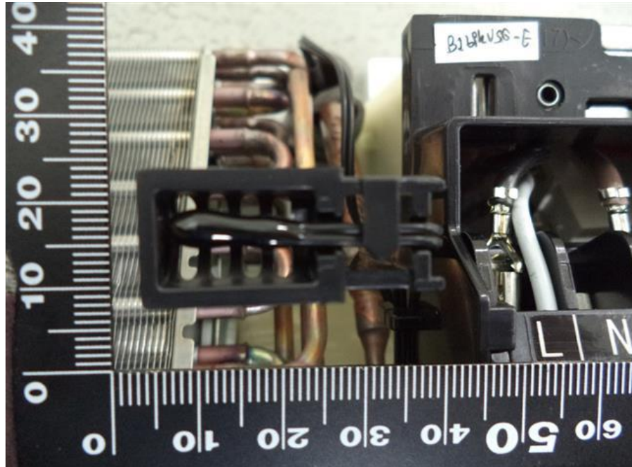
111. RAS-B16PKVSG-E, Thermistor
