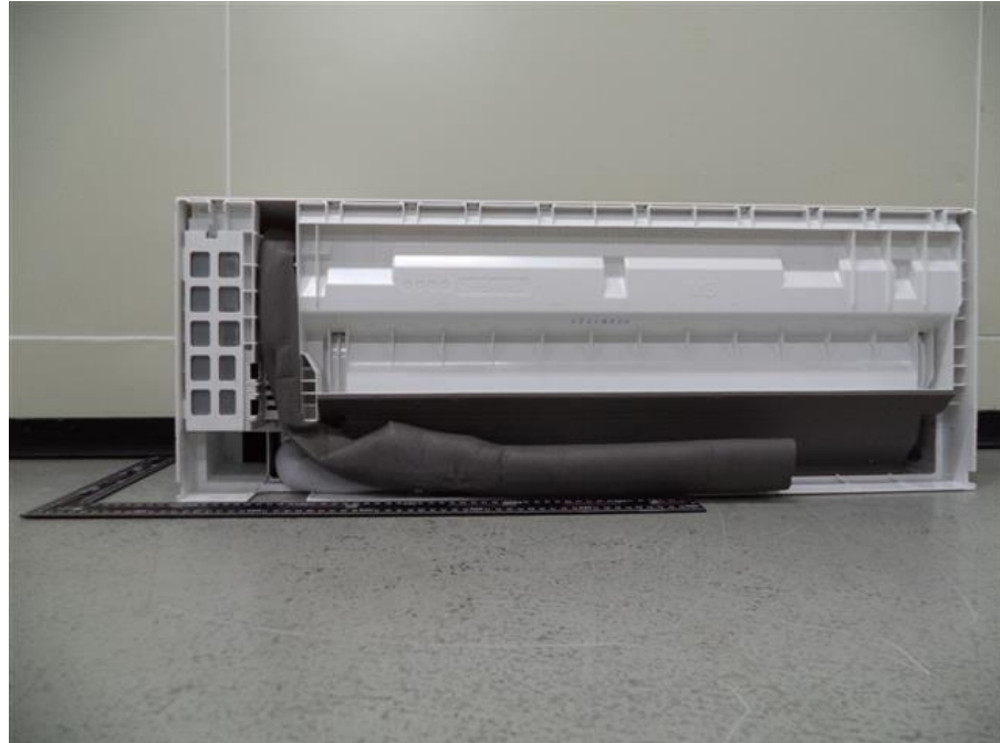
5. RAS-B10PKVSG-E, Rear view removed mounting plate
