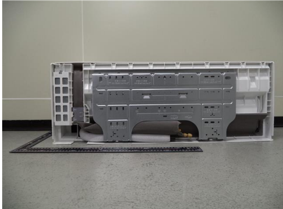
57. RAS-B07BKVG-E, Rear view
