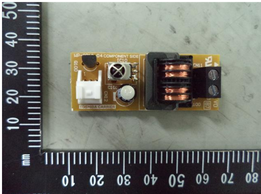
48. RAS-M10PKVPG-E, Receiver board component side
