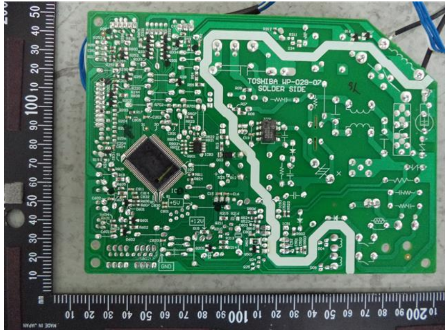
97. RAS-B16BKVGE, Main PCB soldering side
