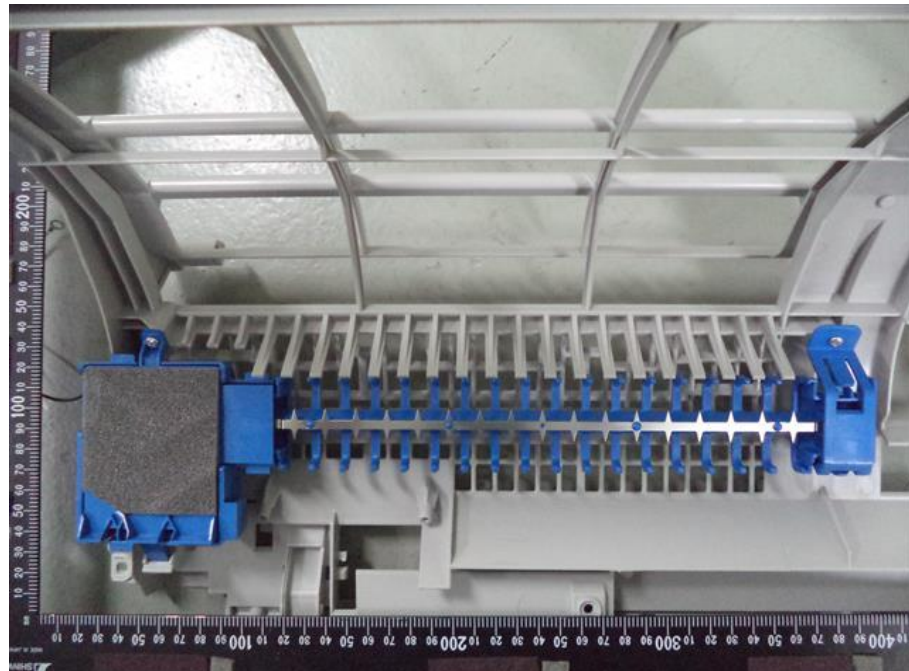
50. RAS-M10PKVPG-E, HV Generator
