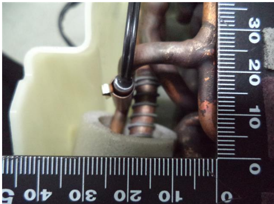
38. RAS-M10PKVPG-E, Thermistor
