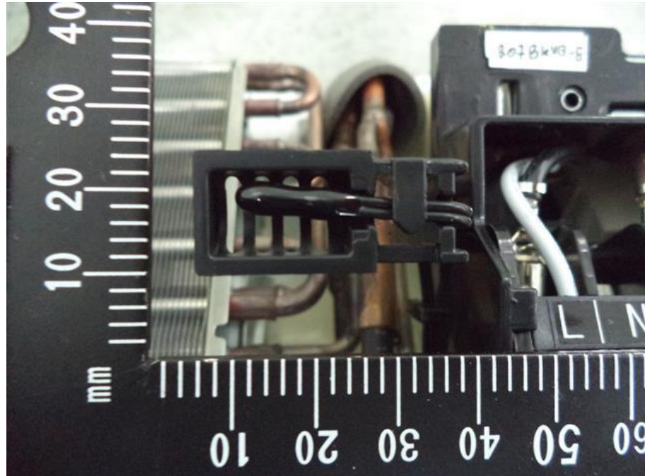
65. RAS-B07BKVG-E, Thermistor
