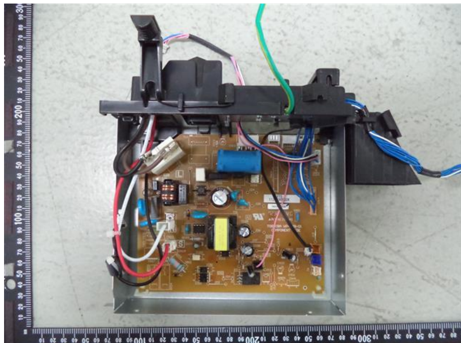
118. RAS-B16PKVSG-E, Electrical control
