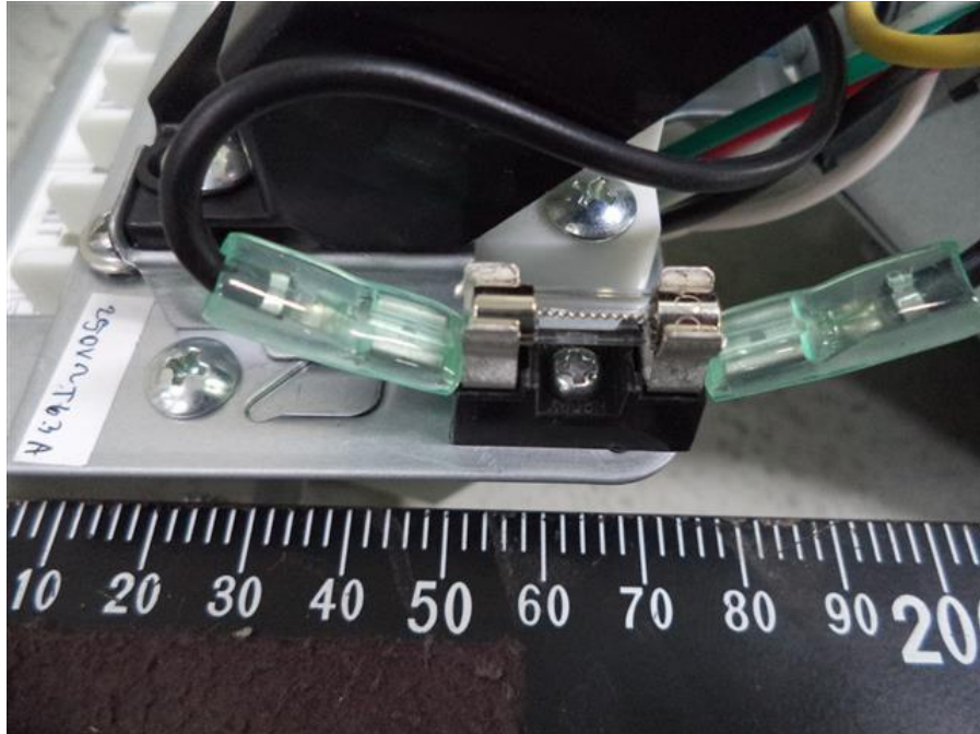
201. RAS-2M10U2AVG-E, RAS-2M14U2AVG-E, RAS-3M18U2AVG-E, Fuse and fuse holder
