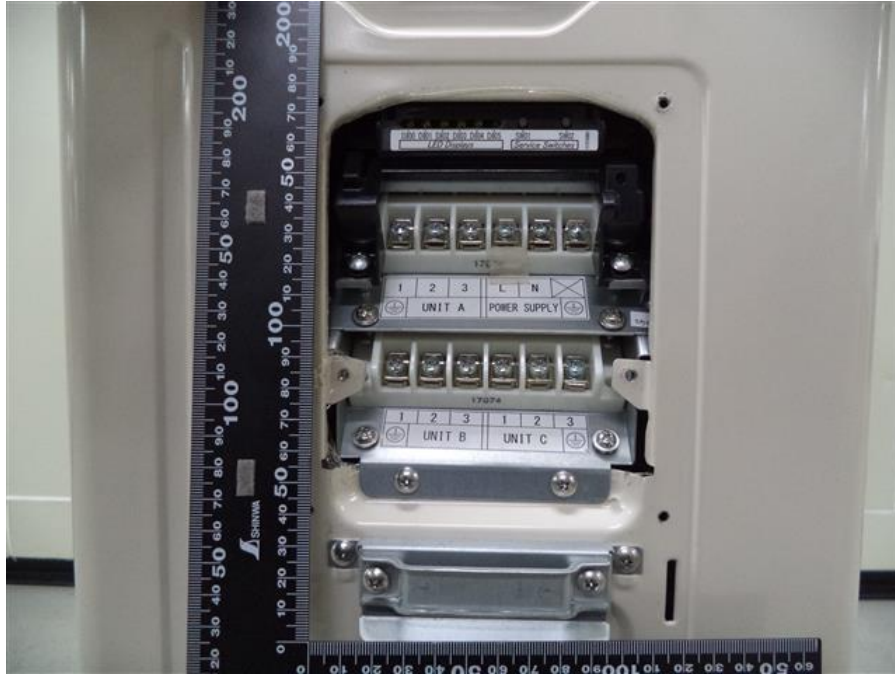
187. RAS-3M18U2AVG-E, Terminal block for interconnecting cable and cord anchorage
