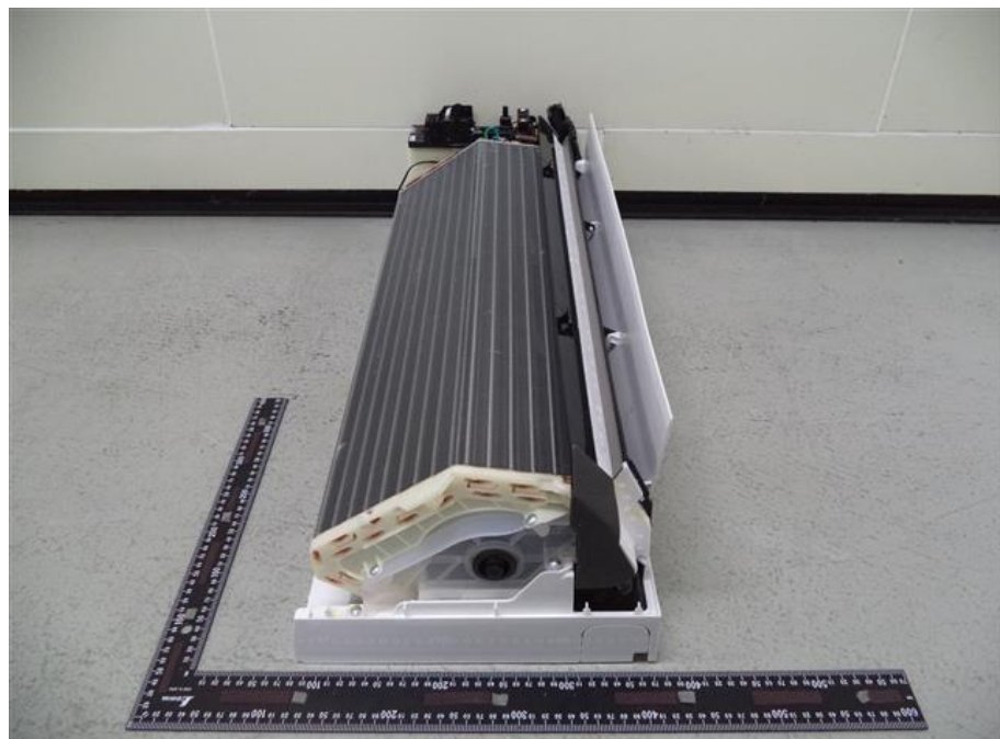
110. RAS-B16PKVSG-E, Internal left view
