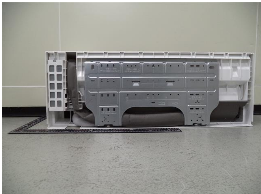
4. RAS-B10PKVSG-E, Rear view
