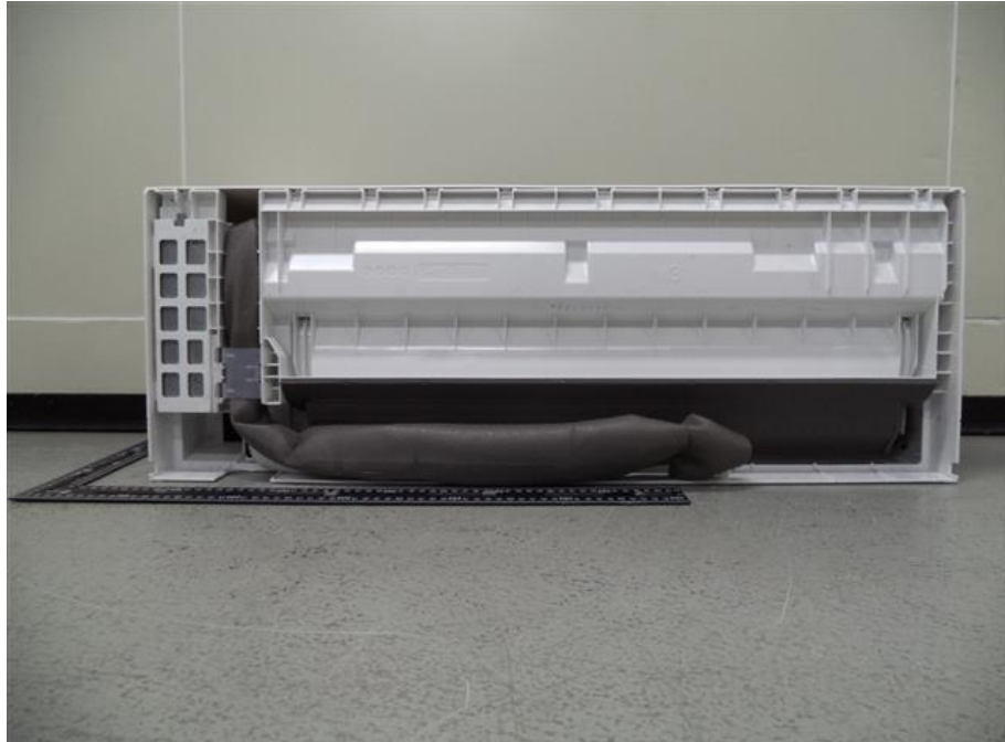
81. RAS-B16BKVG-E, Rear view removed mounting plate
