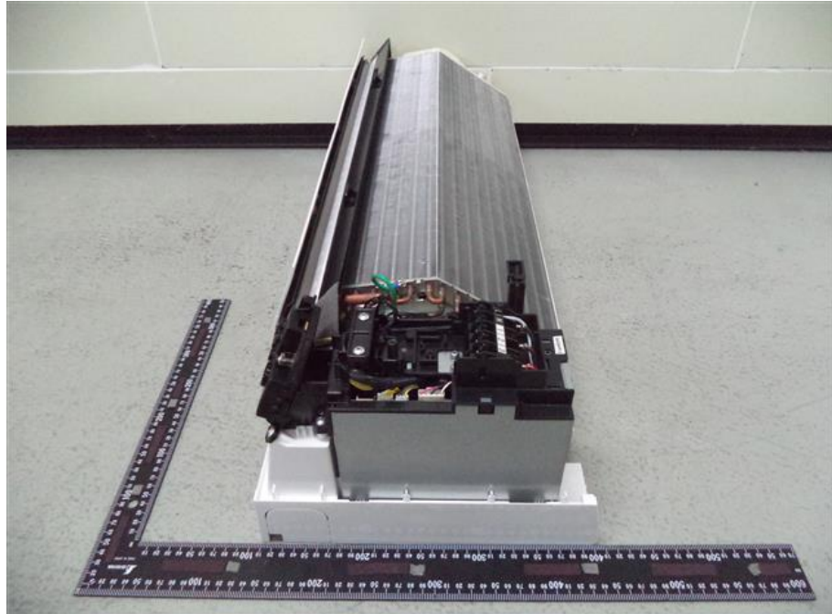
63. RAS-B07BKVG-E, Internal right view
