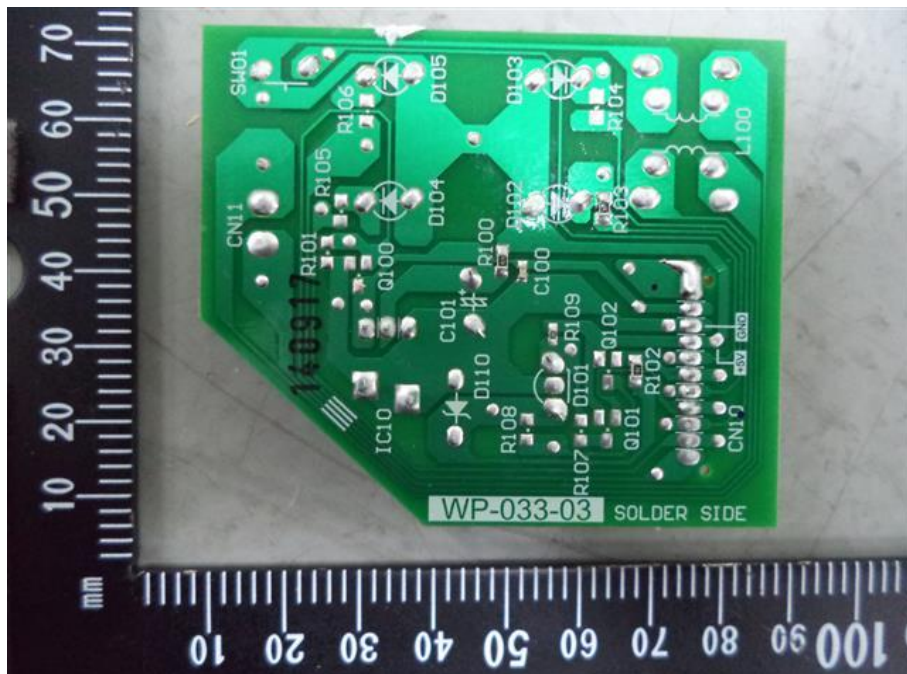
76. RAS-B07BKVG-E, Receiver board solder side
