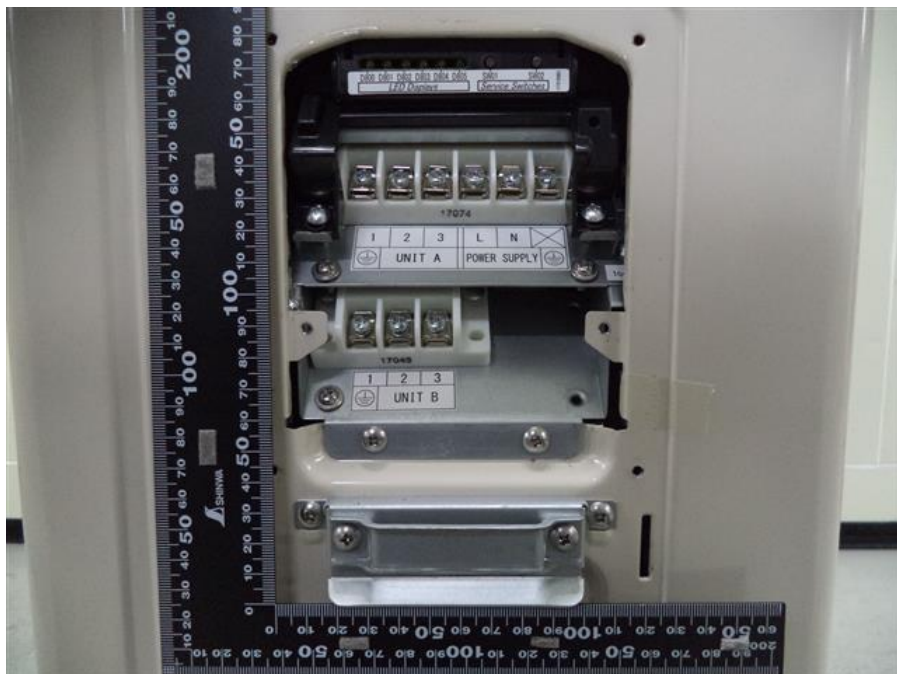
136. RAS-2M10U2AVG-E, Terminal block for interconnecting cable and cord anchorage
