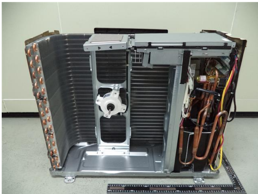
160. RAS-2M14U2AVG-E, Internal view removed fan blade
