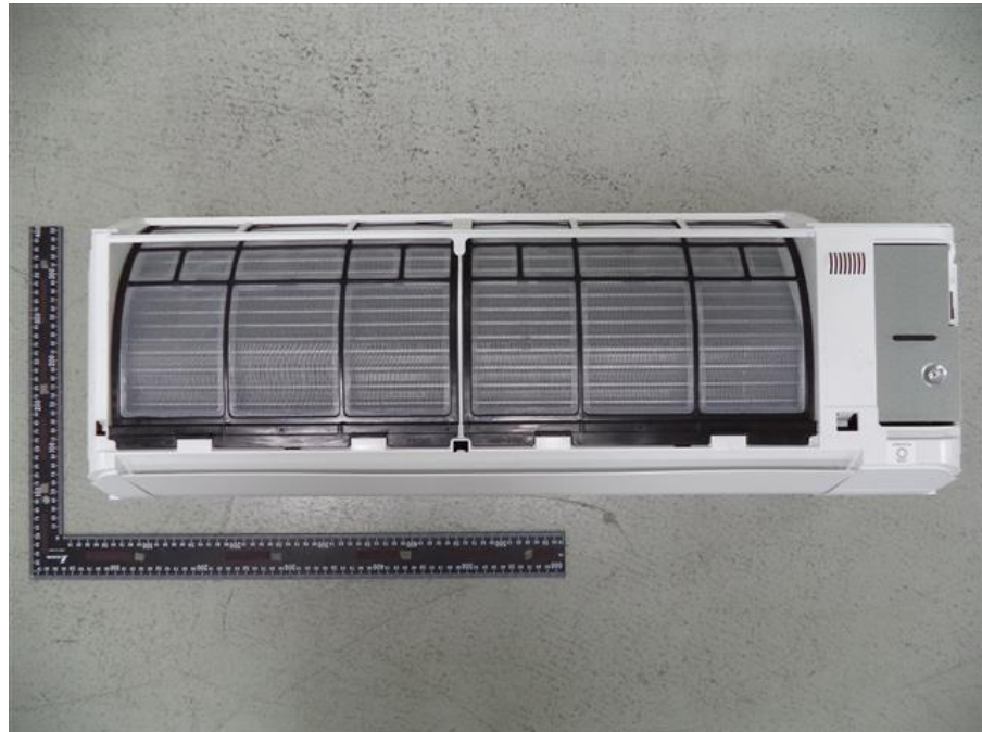
7. RAS-B10PKVSG-E, Front view removed front cover
