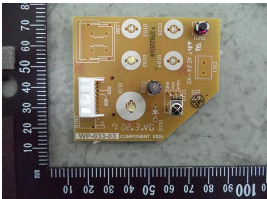
98. RAS-B16BKVGE, Receiver board component side
