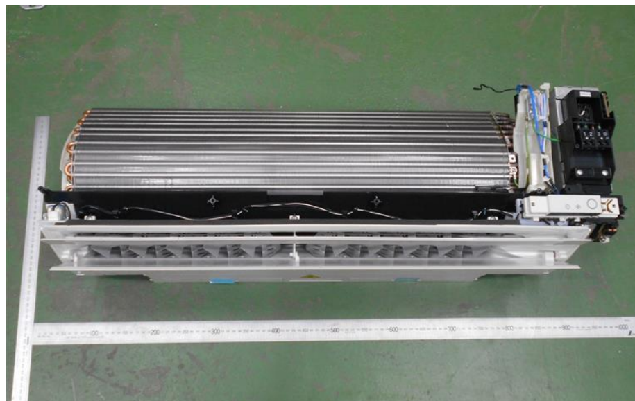
32. RAS-M10PKVPG-E, Internal construction
