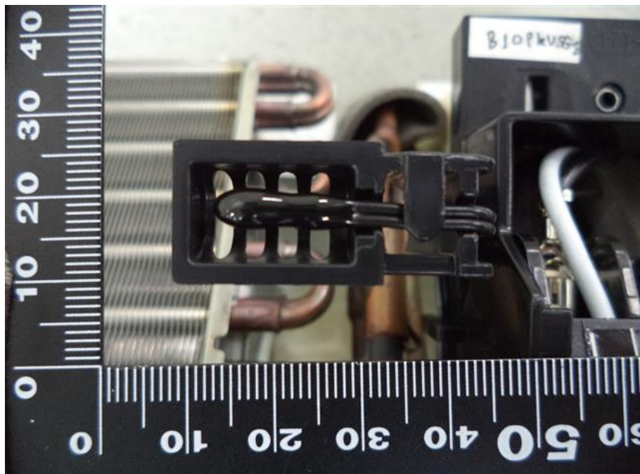
12. RAS-B10PKVSG-E, Thermistor
