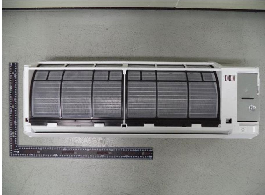
83. RAS-B16BKVGE, Front view removed front cover
