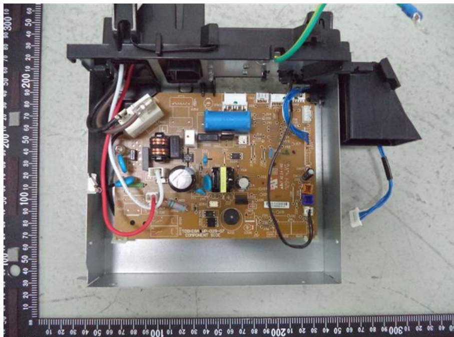
72. RAS-B07BKVG-E, Electrical control
