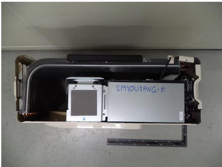
132. RAS-2M10U2AVG-E, Top view removed insulator
