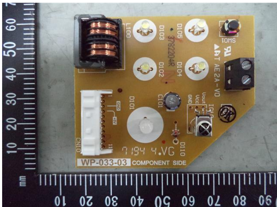
22. RAS-B10PKVSG-E, Receiver board component side
