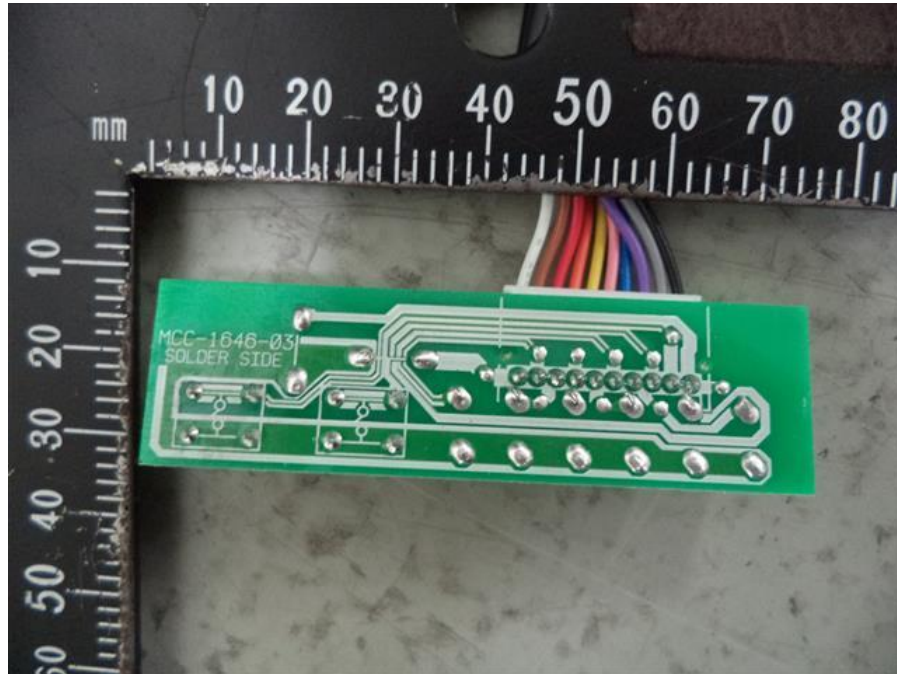
209. RAS-2M10U2AVG-E, RAS-2M14U2AVG-E, RAS-3M18U2AVG-E, MCC-1646, trace side
