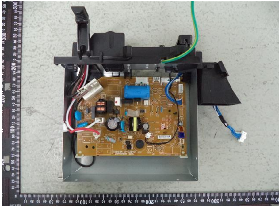
95. RAS-B16BKVG-E, Electrical control
