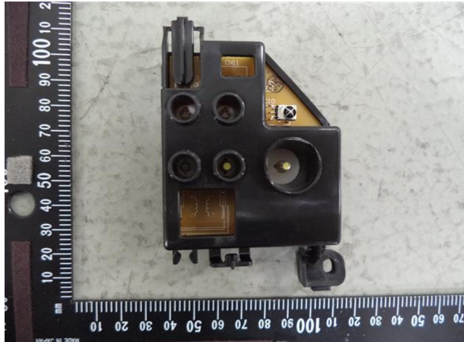
89. RAS-B16BKVG-E, receiver and display
