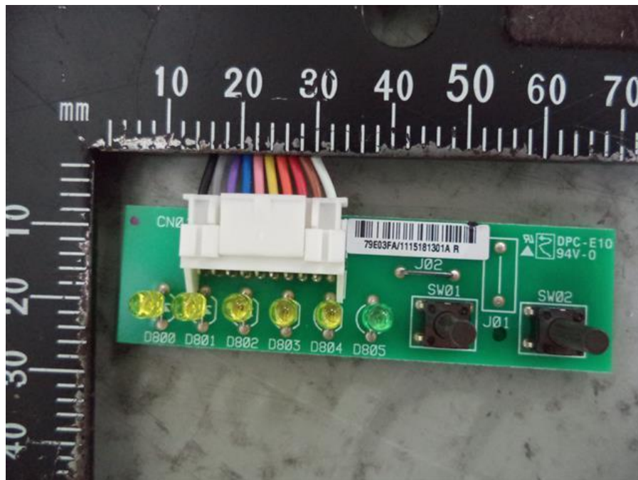
208. RAS-2M10U2AVG-E, RAS-2M14U2AVG-E, RAS-3M18U2AVG-E, MCC-1646, component side
