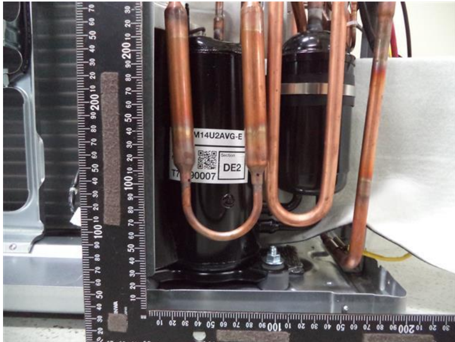
163. RAS-2M14U2AVG-E, Motor compressor
