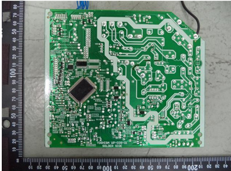
21. RAS-B10PKVSG-E, Main PCB soldering side
