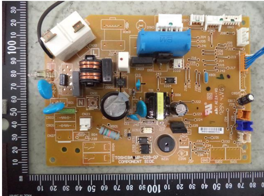
73. RAS-B07BKVG-E, Main PCB component side
