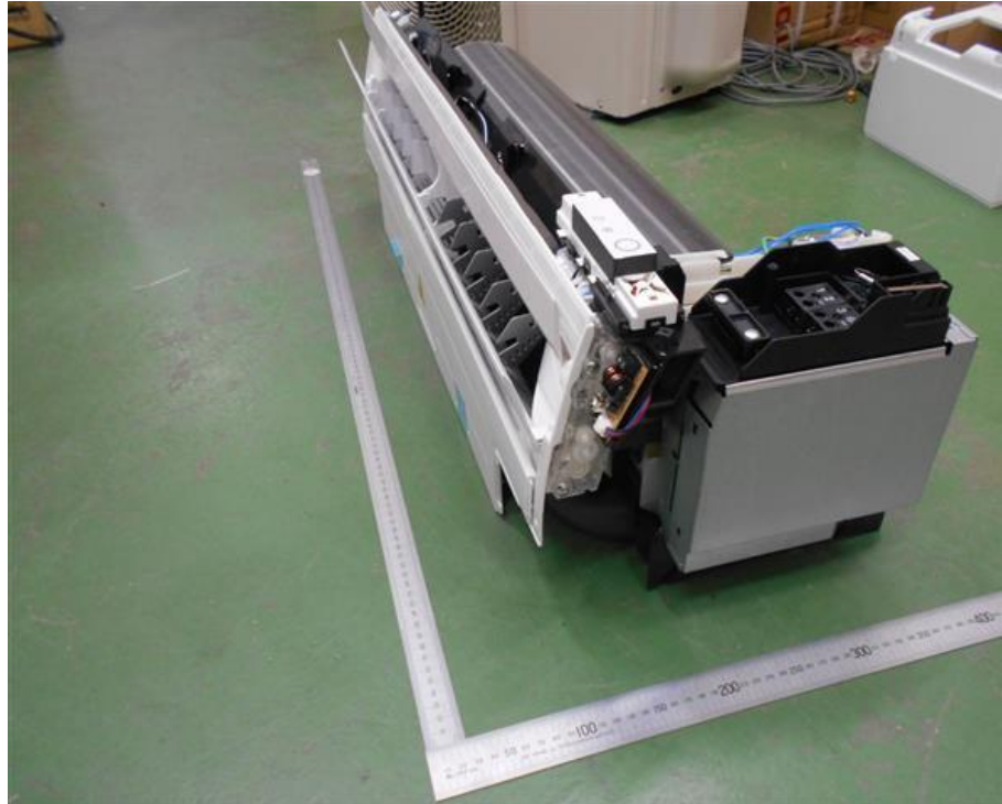
33. RAS-M10PKVPG-E, Internal right view
