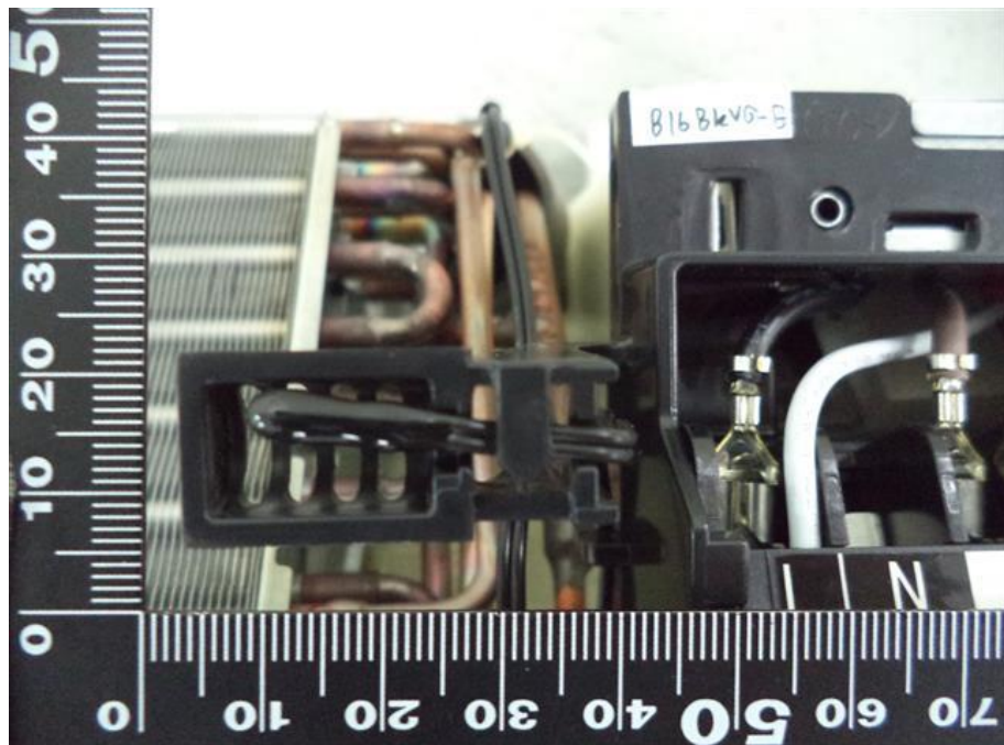
88. RAS-B16BKVG-E, Thermistor
