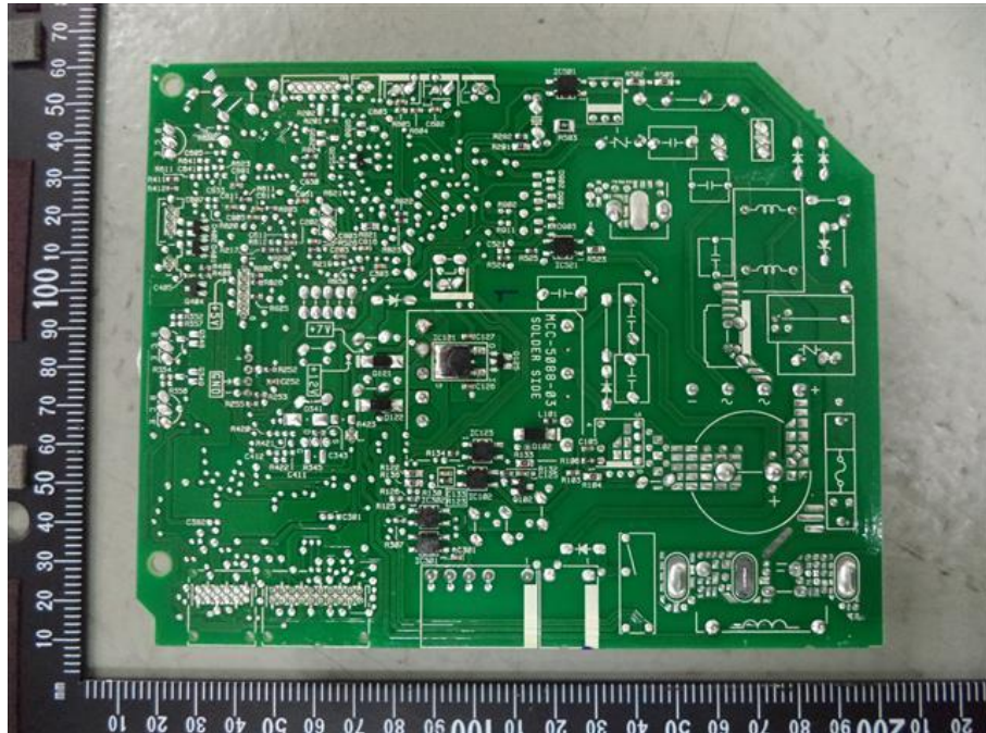
45. RAS-M10PKVPG-E, Main PCB soldering side
