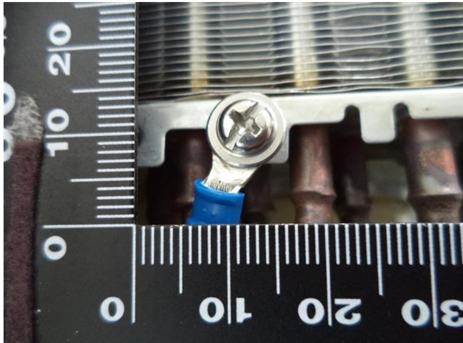
16. RAS-B10PKVSG-E, Earth connection
