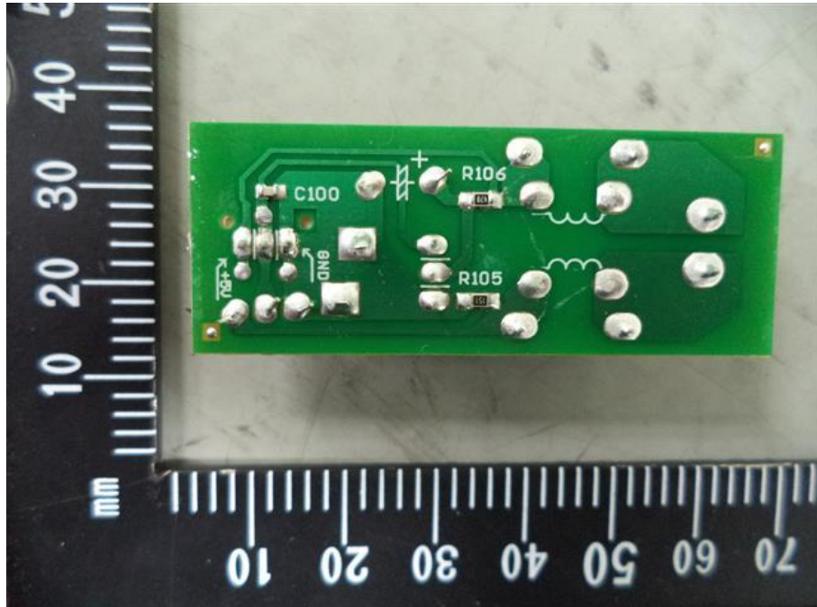
49. RAS-M10PKVPG-E, Receiver board solder side
