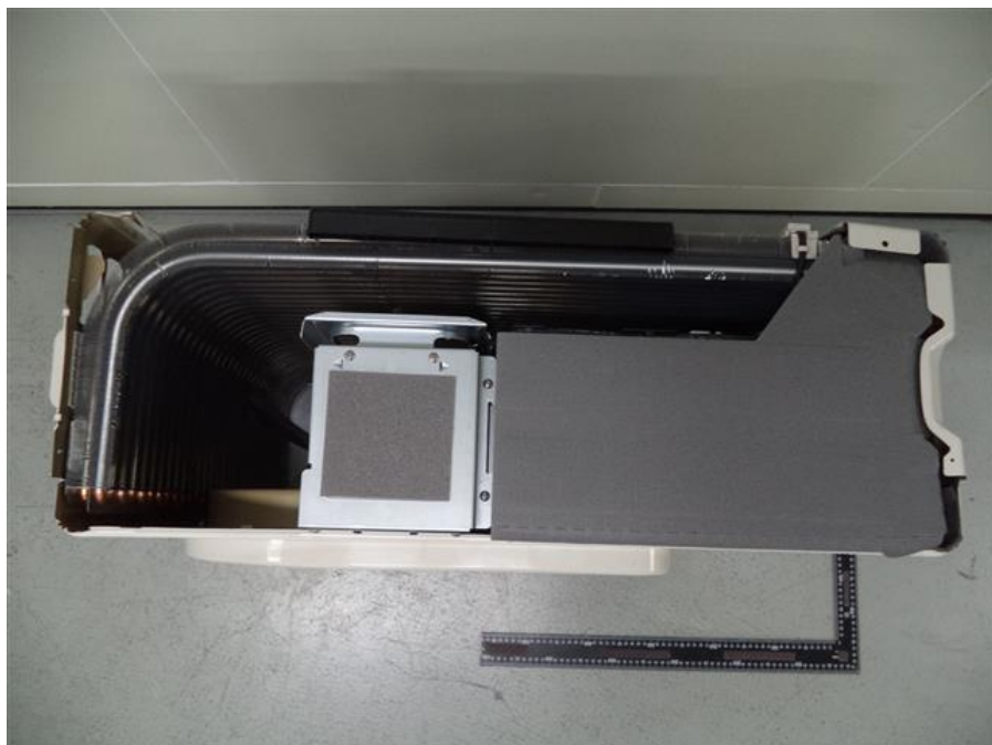
156. RAS-2M14U2AVG-E, Top view removed top cover
