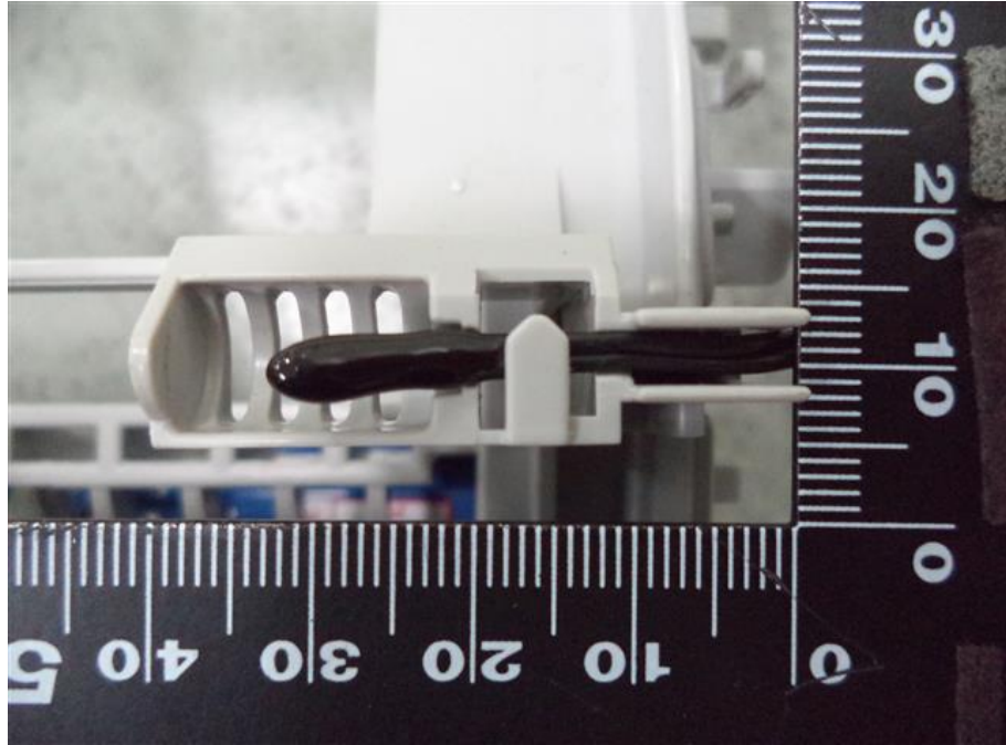
35. RAS-M10PKVPG-E, Thermistor
