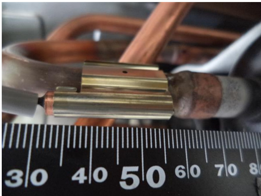
196. RAS-3M18U2AVG-E, Thermistor
