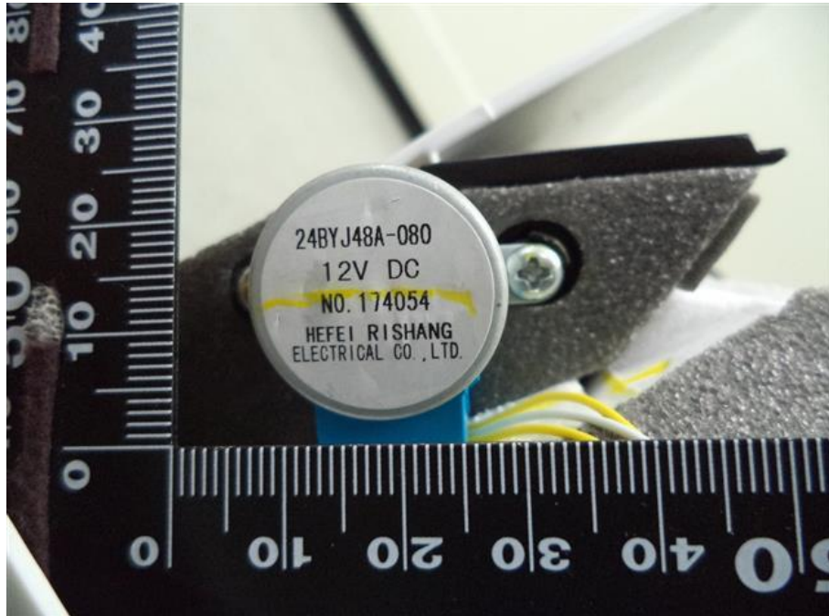
71. RAS-B07BKVG-E, Louver motor (Vertical)
