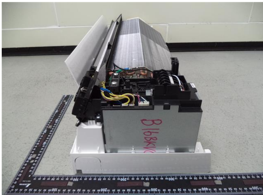
86. RAS-B16BKVG-E, Internal right view
