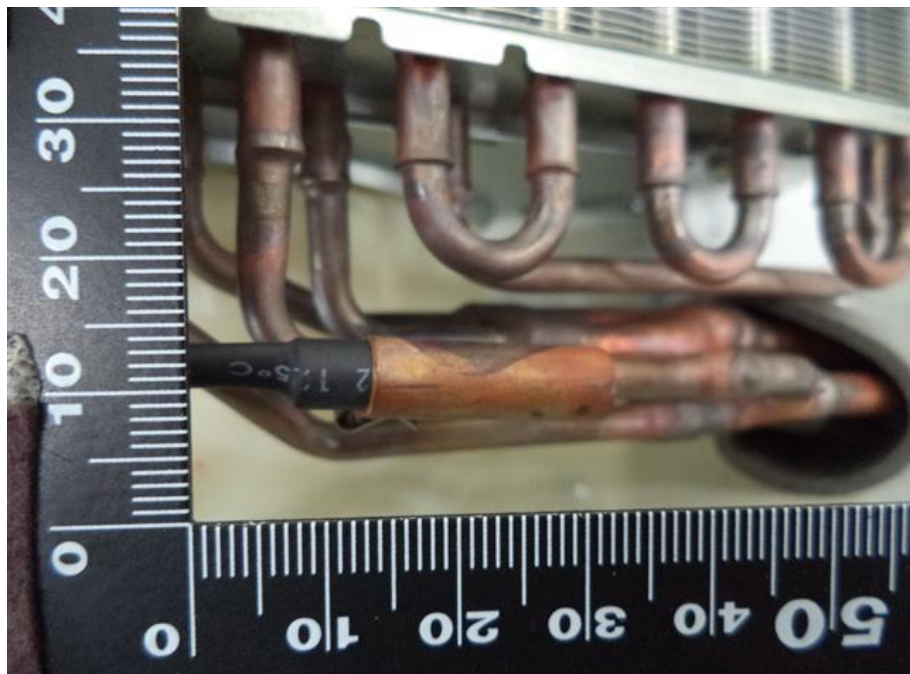
68. RAS-B07BKVG-E, Thermistor
