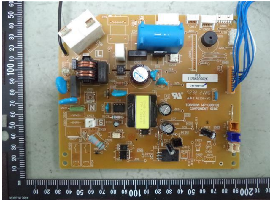
119. RAS-B16PKVSG-E, Main PCB component side
