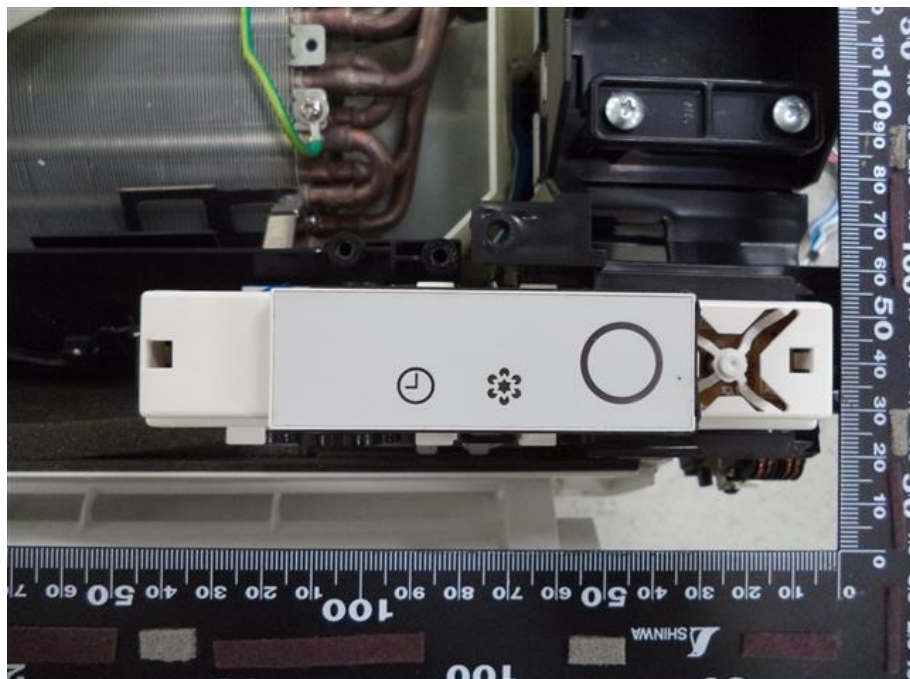
36. RAS-M10PKVPG-E, receiver and display
