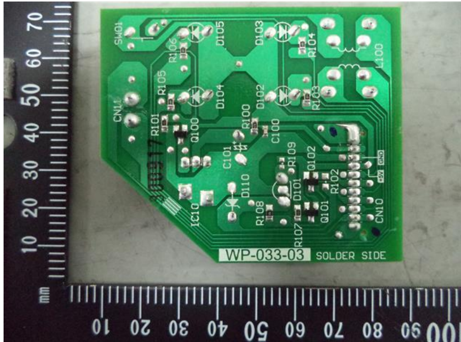
23. RAS-B10PKVSG-E, Receiver board solder side
