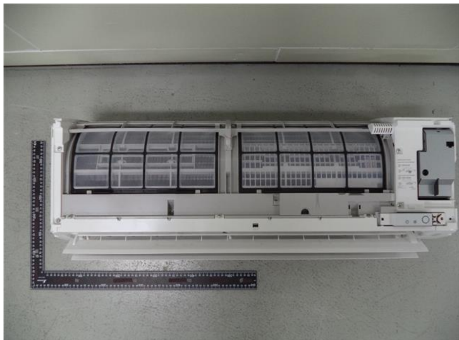
30. RAS-M10PKVPG-E, Front view removed front cover
