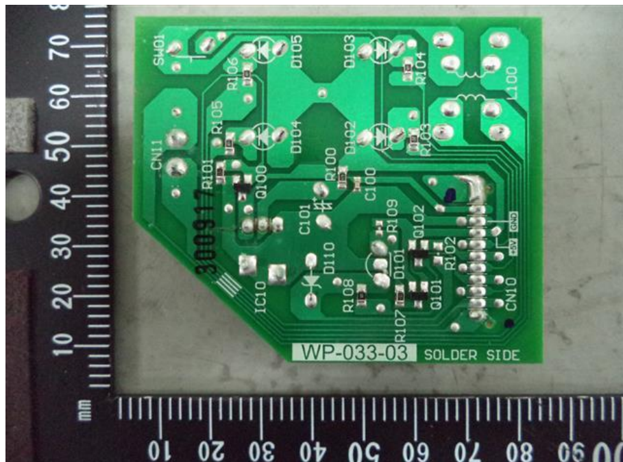
122. RAS-B16PKVSG-E, Receiver board solder side
