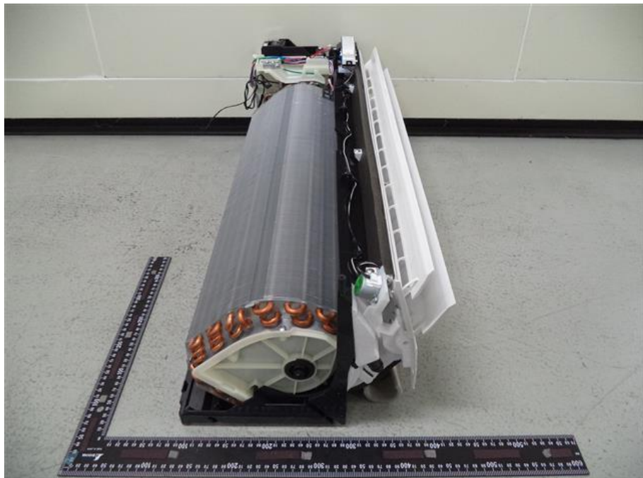
34. RAS-M10PKVPG-E, Internal left view
