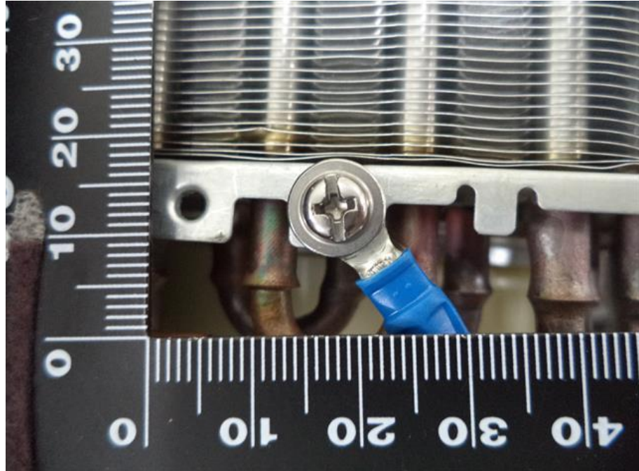
115. RAS-B16PKVSG-E, Earth connection
