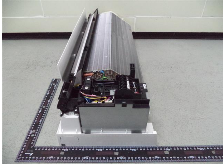
109. RAS-B16PKVSG-E, Internal right view
