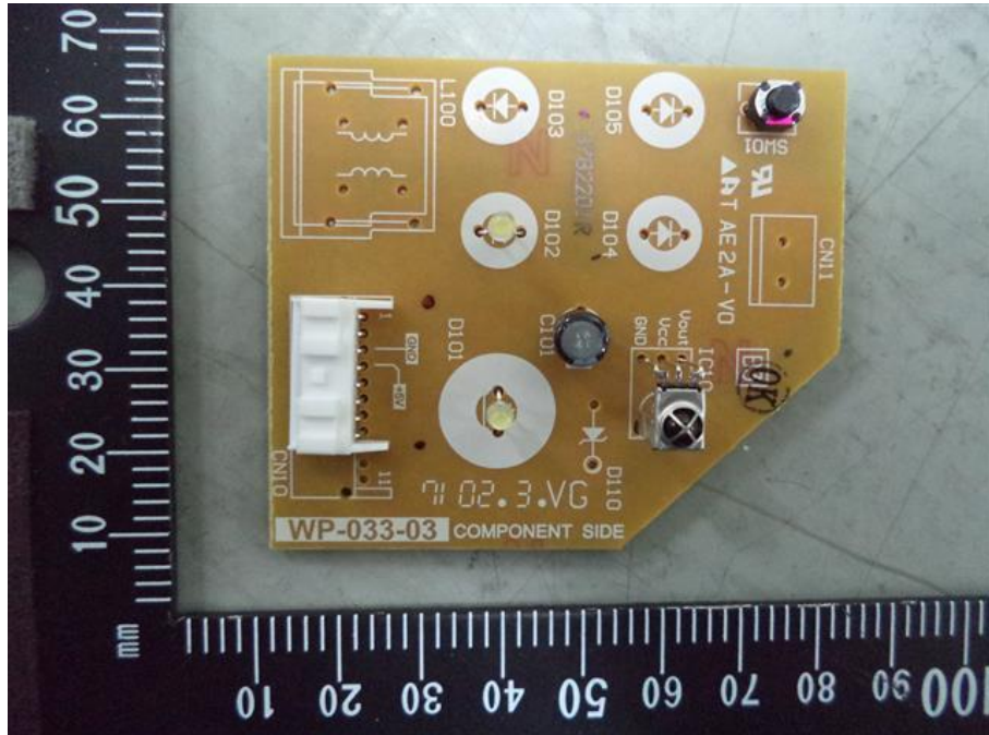
75. RAS-B07BKVG-E, Receiver board component side
