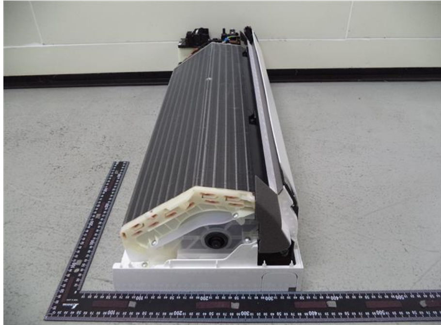
11. RAS-B10PKVSG-E, Internal left view
