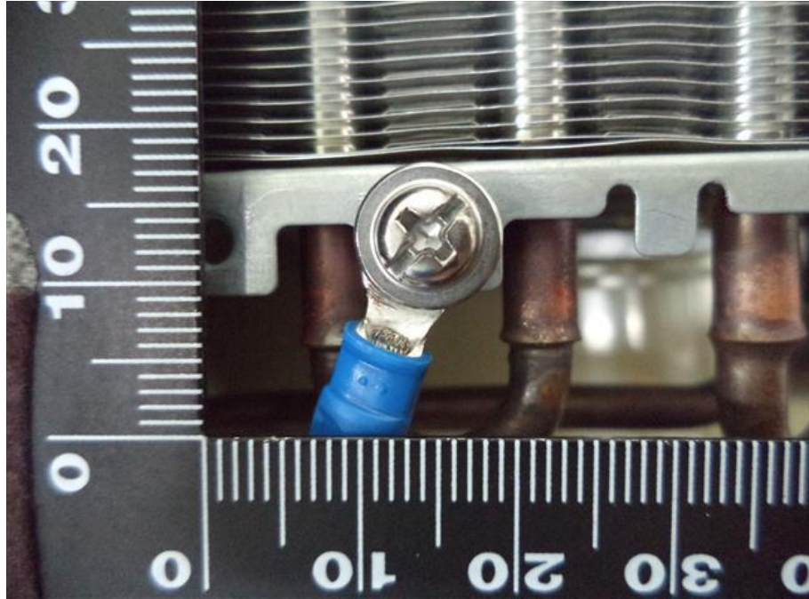
69. RAS-B07BKVG-E, Earth connection
