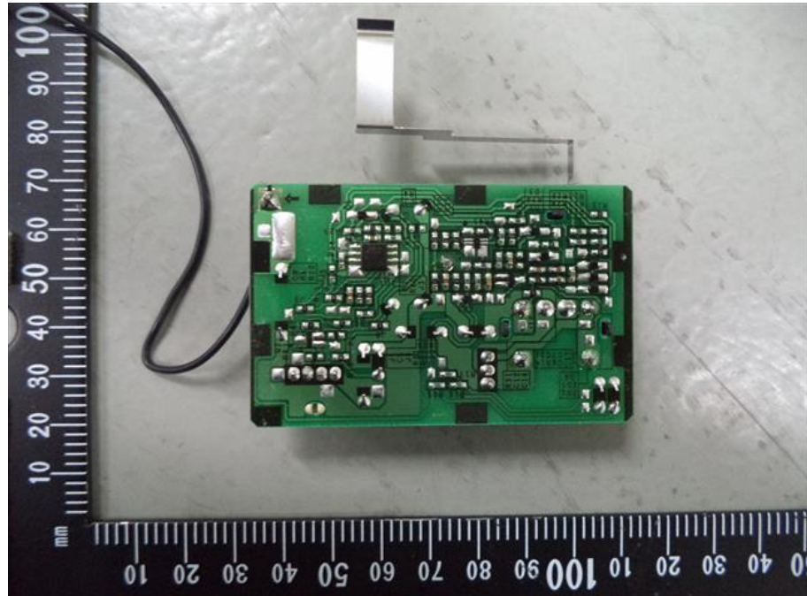
53. RAS-M10PKVPG-E, HV Generator trace side
