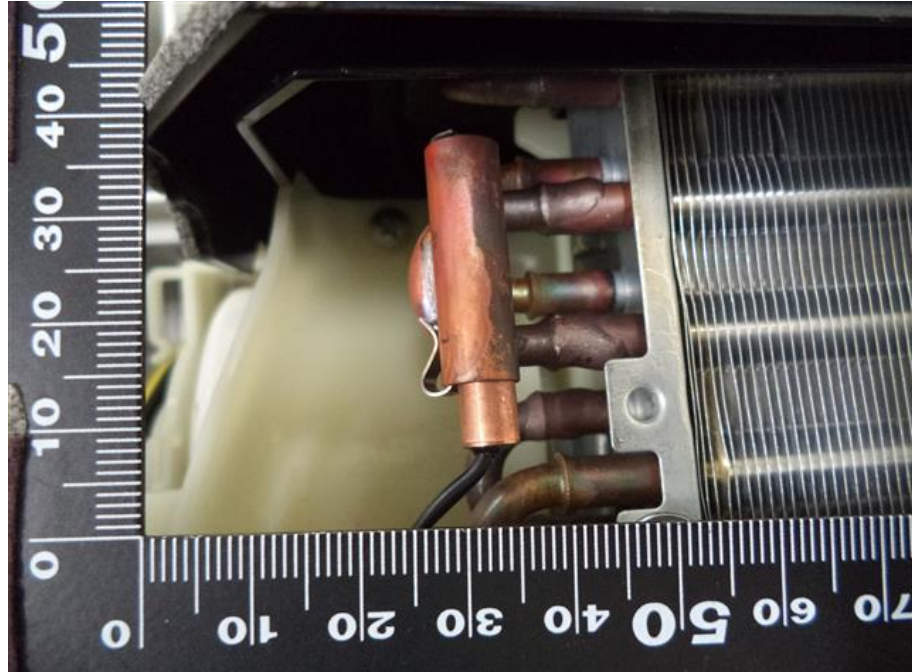
113. RAS-B16PKVSG-E, Thermistor
