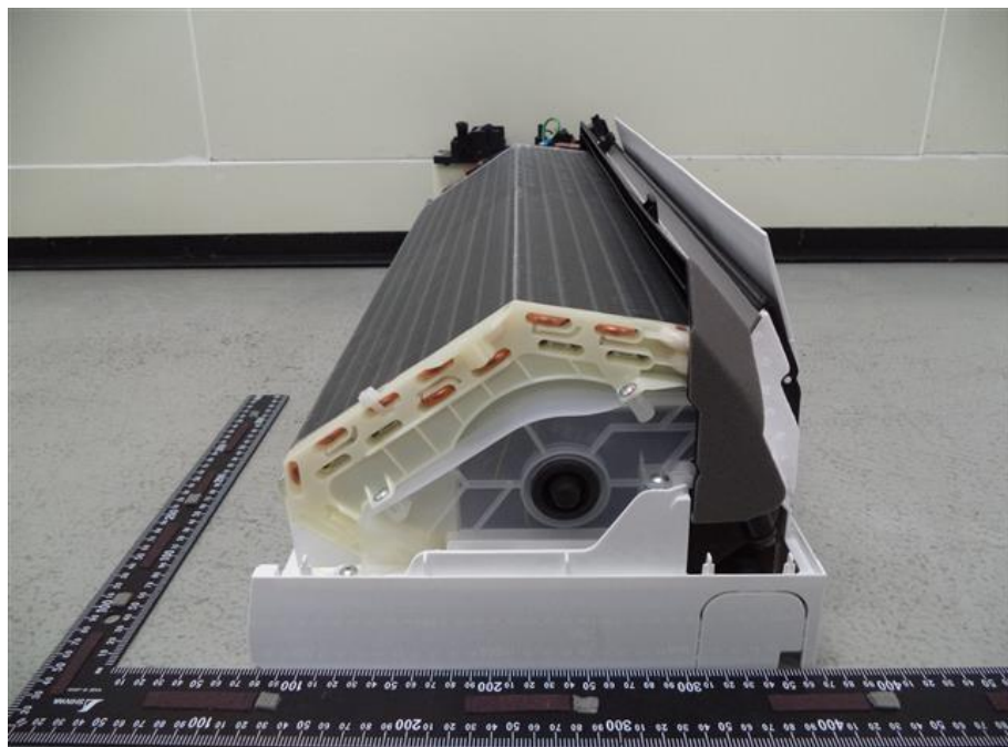
64. RAS-B07BKVG-E, Internal left view
