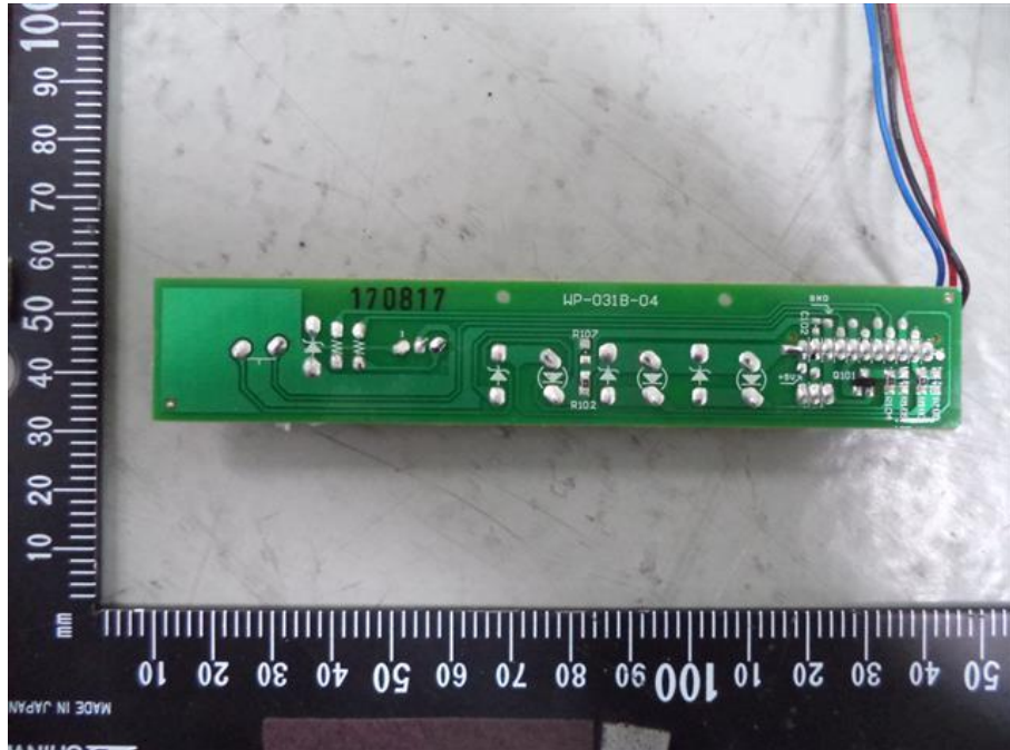
47. RAS-M10PKVPG-E, Display trace side
