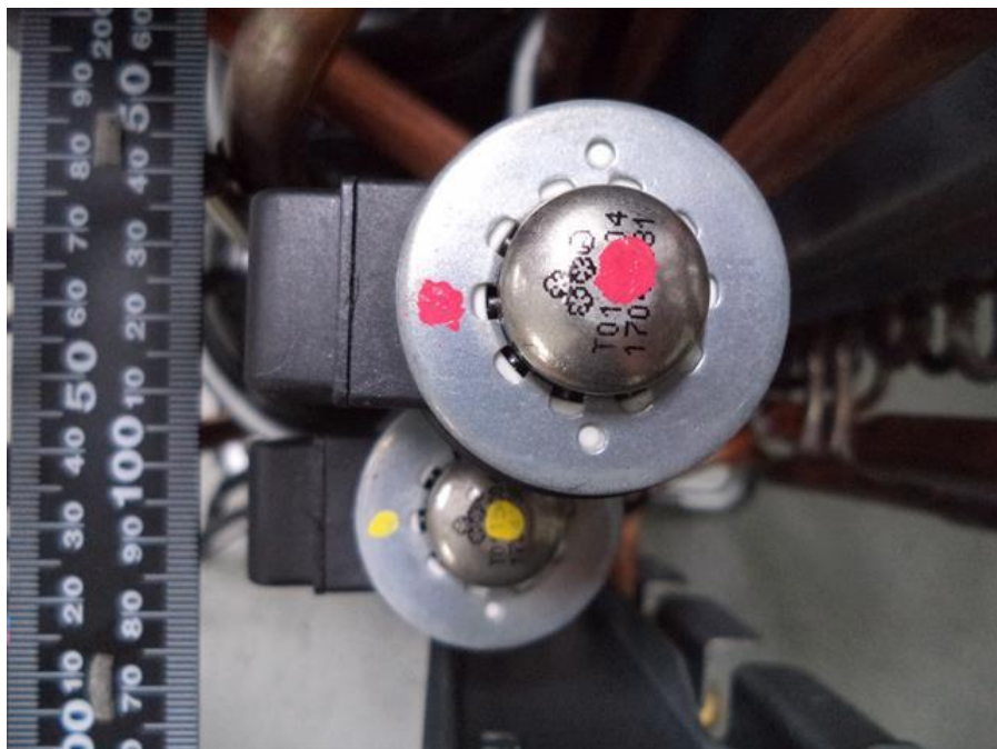
172. RAS-2M14U2AVG-E, PMV Coil
