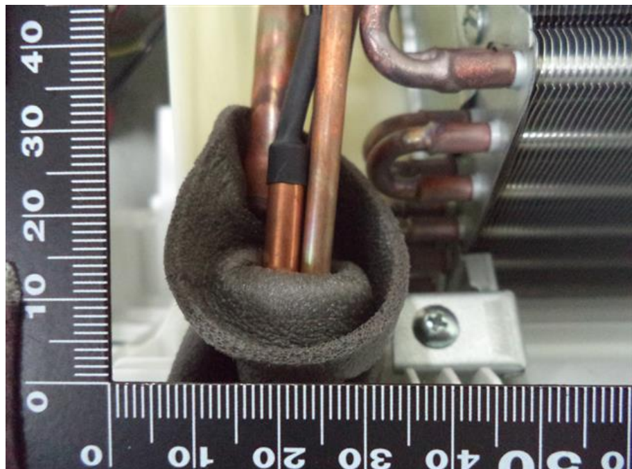
114. RAS-B16PKVSG-E, Thermistor
