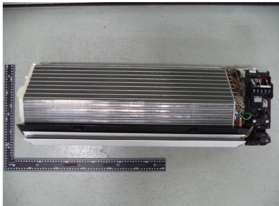
62. RAS-B07BKVG-E, Internal construction
