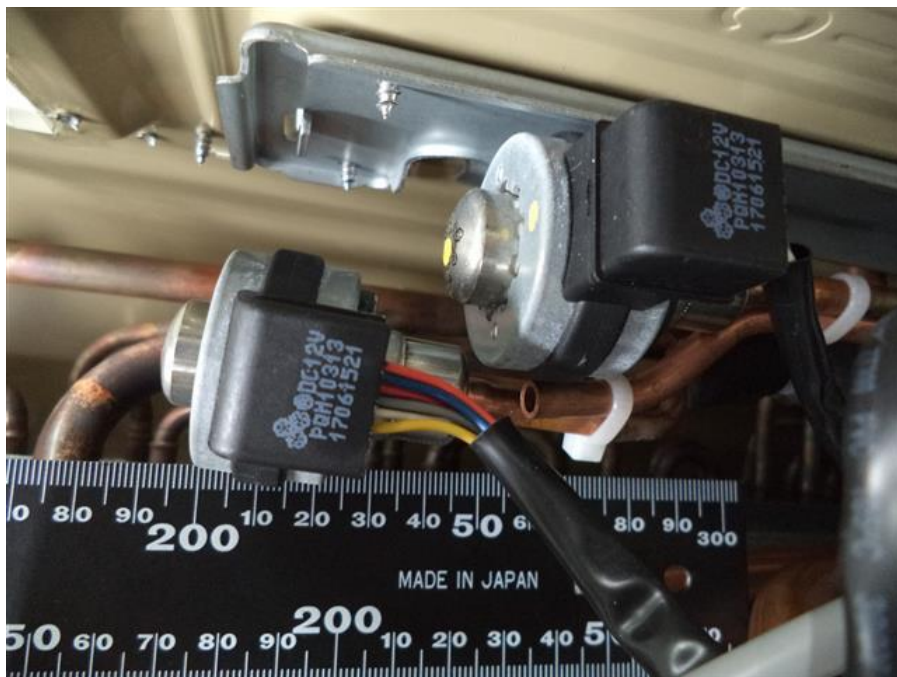
146. RAS-2M10U2AVG-E, PMV Coil
