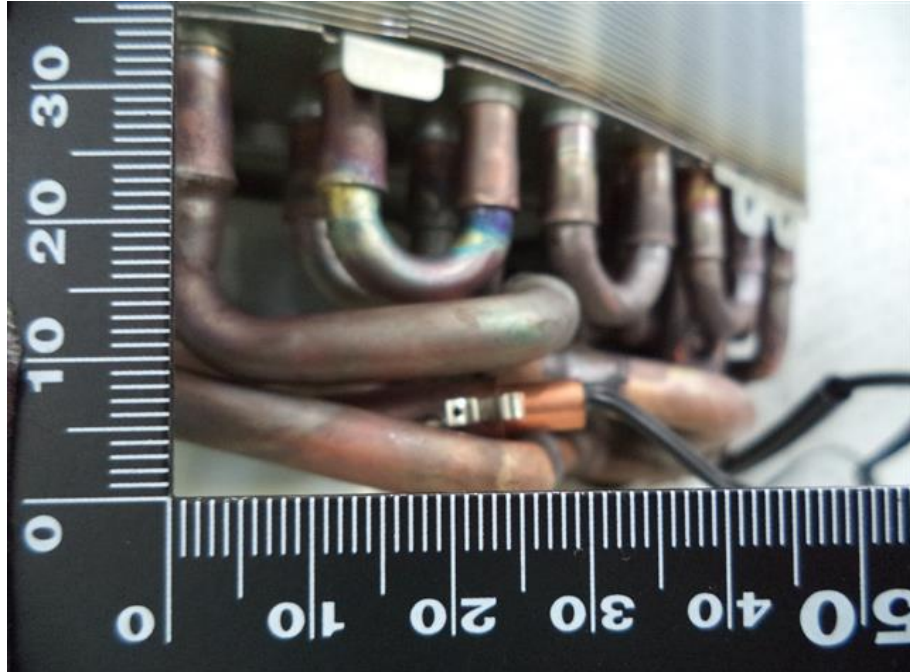
37. RAS-M10PKVPG-E, Thermistor
