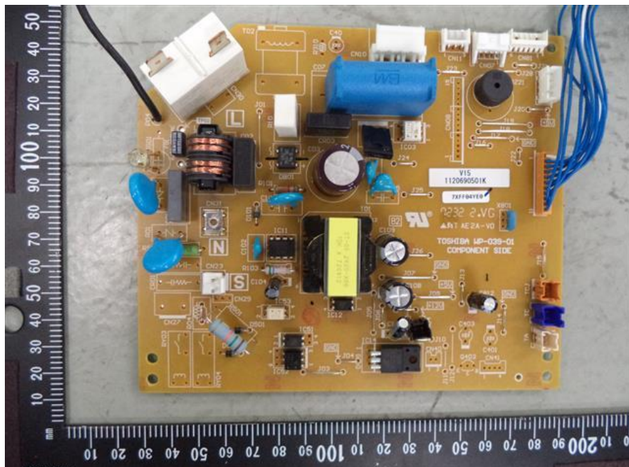
20. RAS-B10PKVSG-E, Main PCB component side
