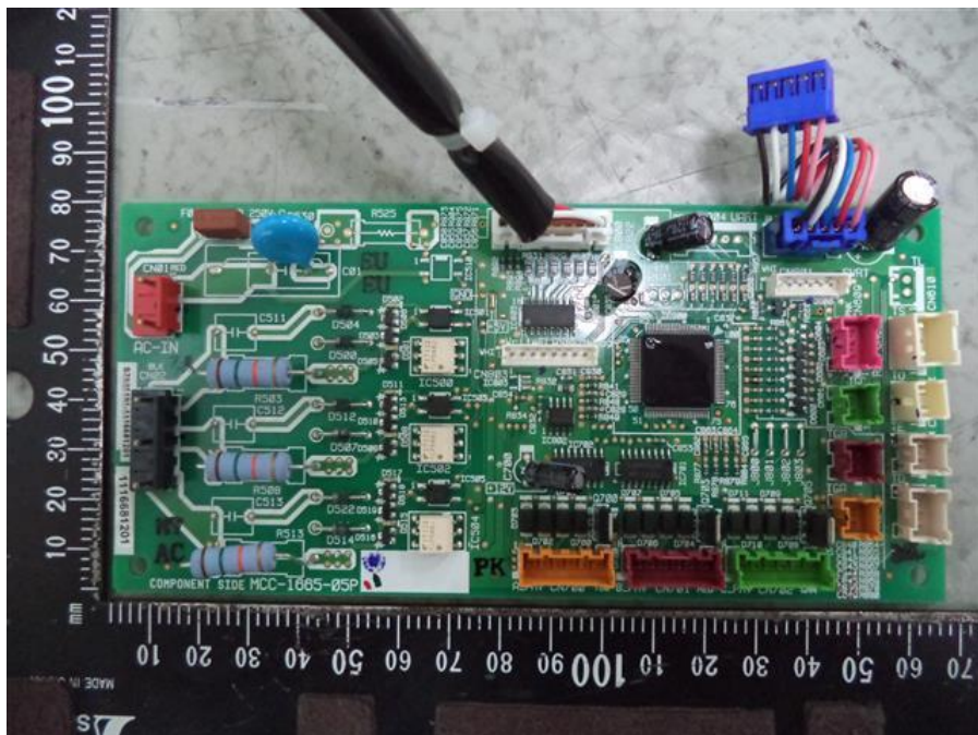
206. RAS-2M10U2AVG-E, RAS-2M14U2AVG-E, RAS-3M18U2AVG-E, MCC-1665, component site
