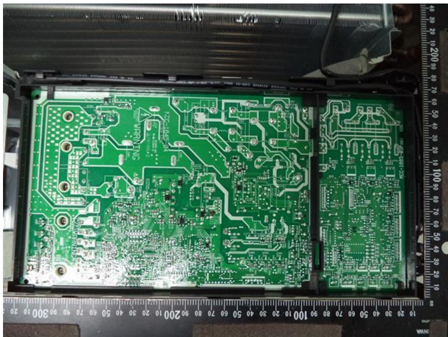
188. RAS-3M18U2AVG-E, Internal construction removed cover
