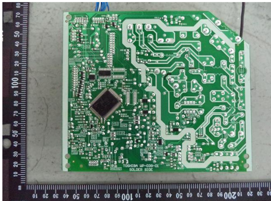
120. RAS-B16PKVSG-E, Main PCB soldering side
