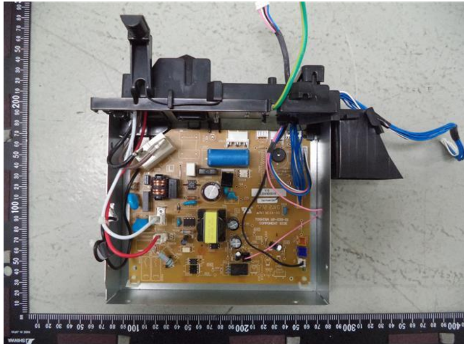
19. RAS-B10PKVSG-E, Electrical control
