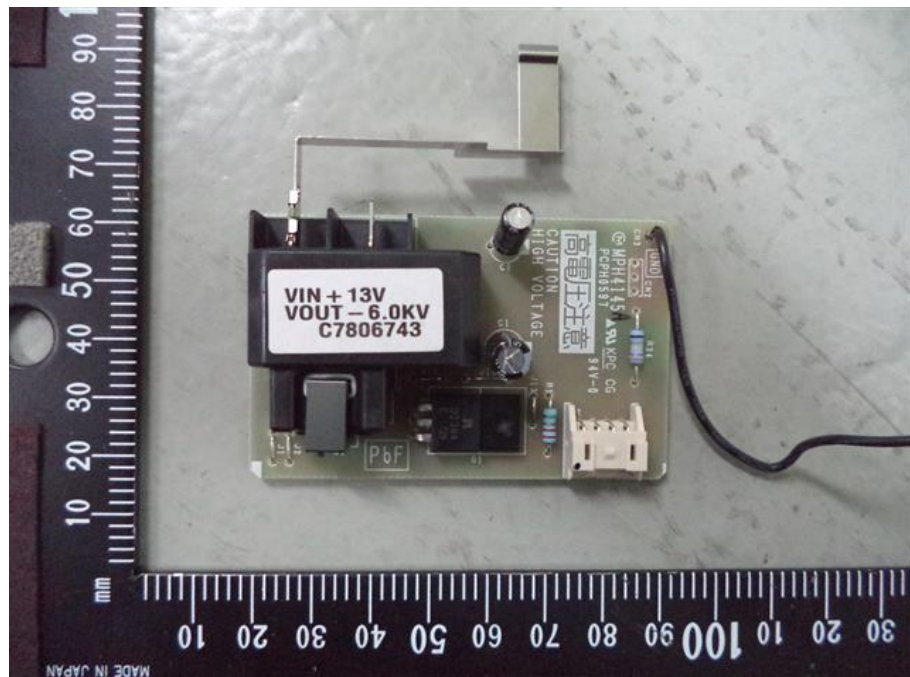
52. RAS-M10PKVPG-E, HV Generator component side
