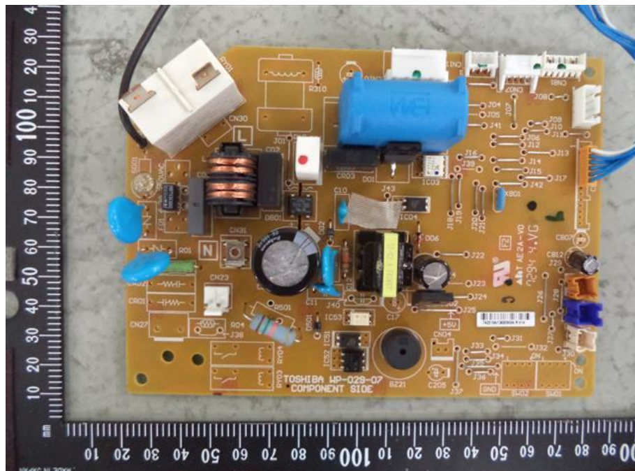
96. RAS-B16BKVG-E, Main PCB component side
