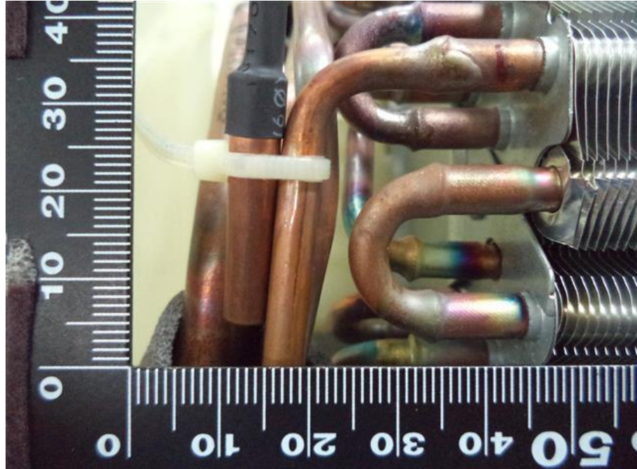
91. RAS-B16BKVG-E, Thermistor
