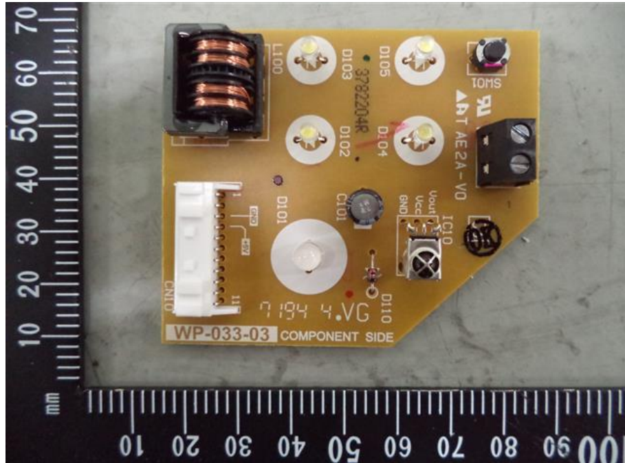
121. RAS-B16PKVSG-E, Receiver board component side
