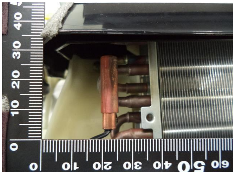
90. RAS-B16BKVG-E, Thermistor
