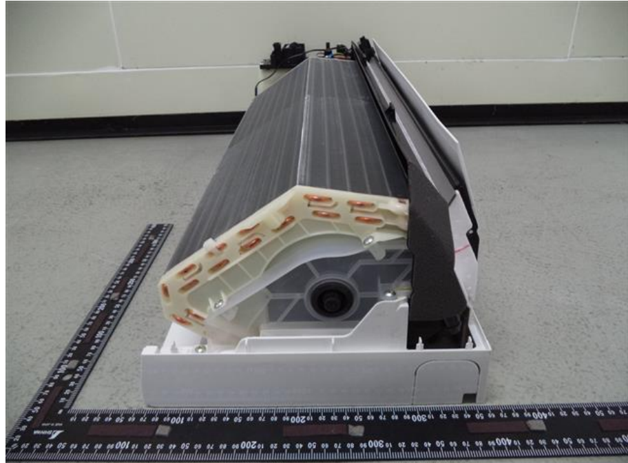
87. RAS-B16BKVG-E, Internal left view
