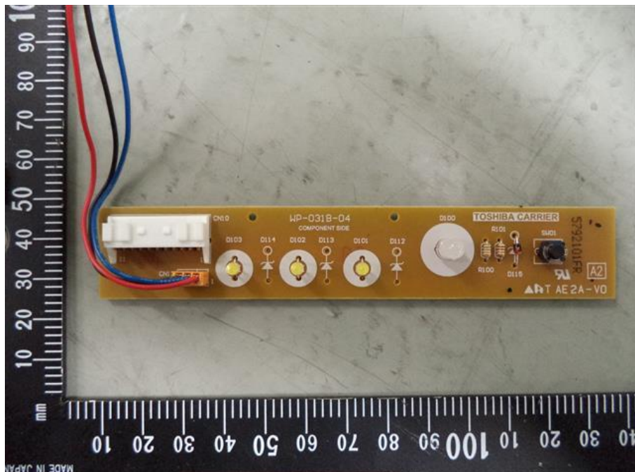
46. RAS-M10PKVPG-E, Display component side
