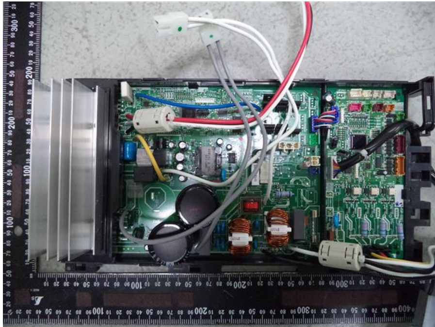
203. RAS-2M10U2AVG-E, RAS-2M14U2AVG-E, RAS-3M18U2AVG-E, Electrical control
