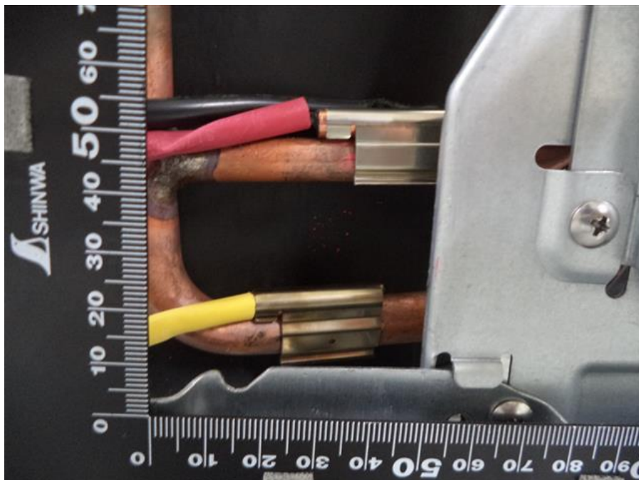
144. RAS-2M10U2AVG-E, Thermistor
