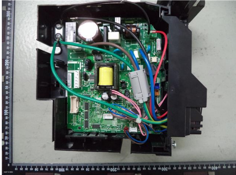
43. RAS-M10PKVPG-E, Electrical control
