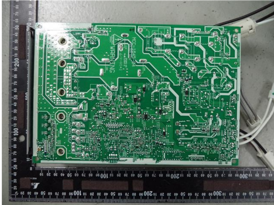
205. RAS-2M10U2AVG-E, RAS-2M14U2AVG-E, RAS-3M18U2AVG-E, MCC-1645, trace side main P.C.B.
