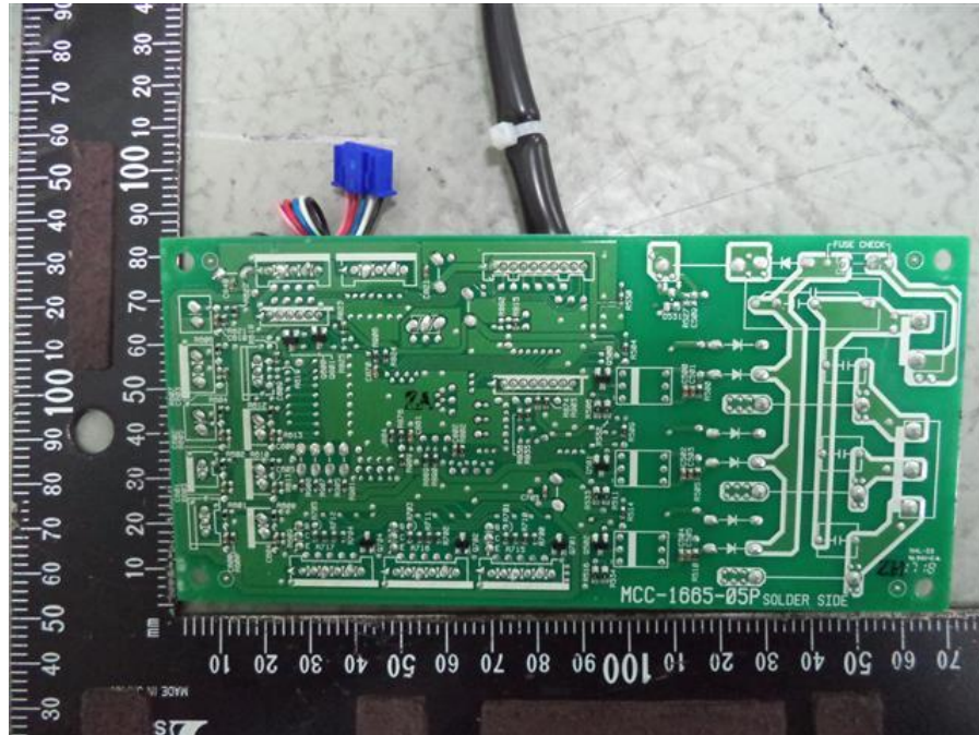
207. RAS-2M10U2AVG-E, RAS-2M14U2AVG-E, RAS-3M18U2AVG-E, MCC-1665, trace side
