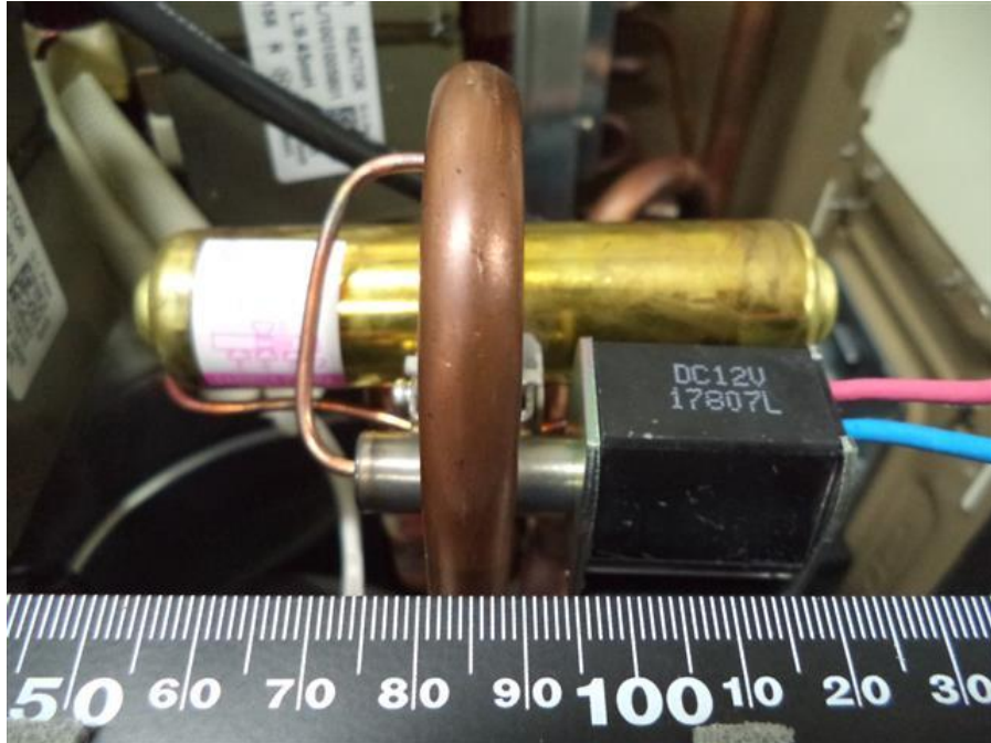
145. RAS-2M10U2AVG-E, 3 Way Valve Coil
